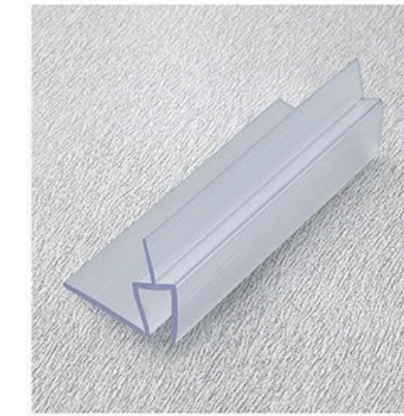
B011BY For 6mm glass
